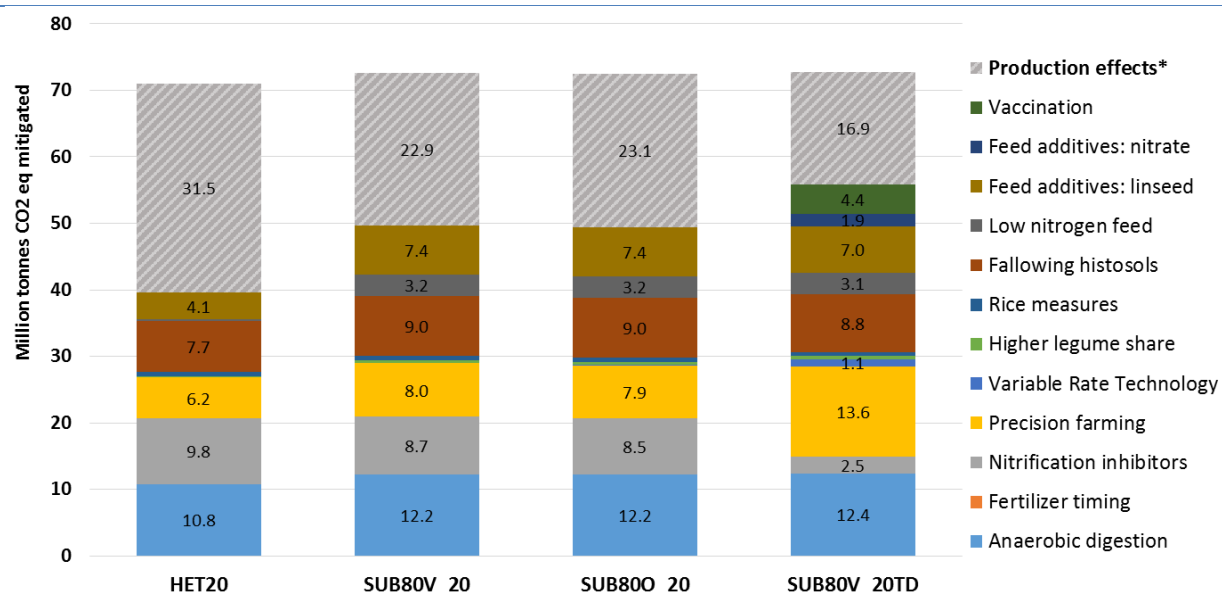
Figure 23: Contribution of each technological mitigation option to total mitigation in the EU-28
