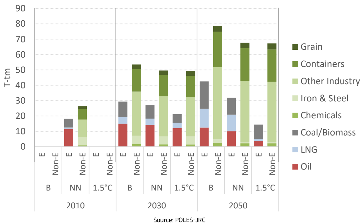
Figure 27: International maritime activity decomposed by type of goods transported
