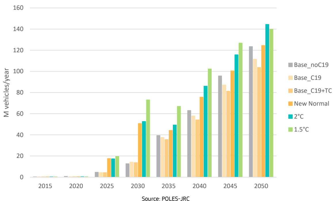
Figure 19: Annual global sales of battery-electric LDVs
